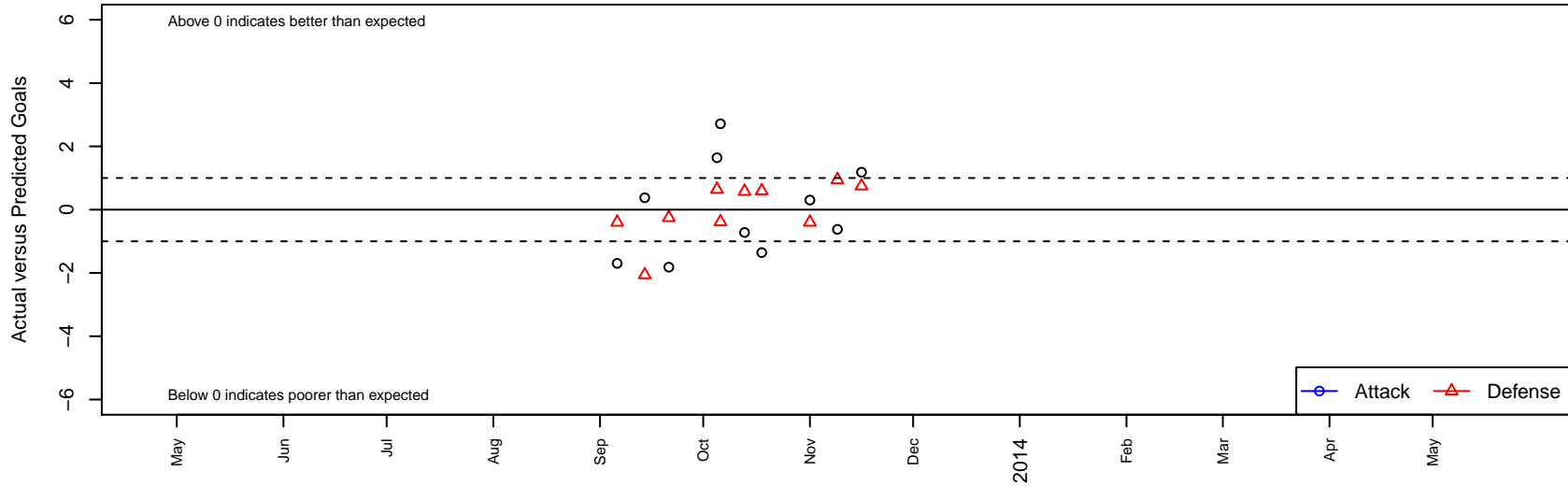
Davis Legacy 03 Strikers G02 Dots are actual minus expected GF (blue circles) and GA (red triangles). Blue line is smoothed change in attack strength. Red is smoothed change in defense strength.
